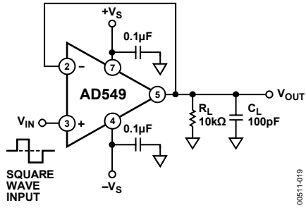
Figure 19. Unity Gain Follower
