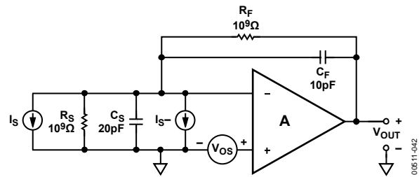
Figure 42. Photodiode Preamp DC Error Sources
